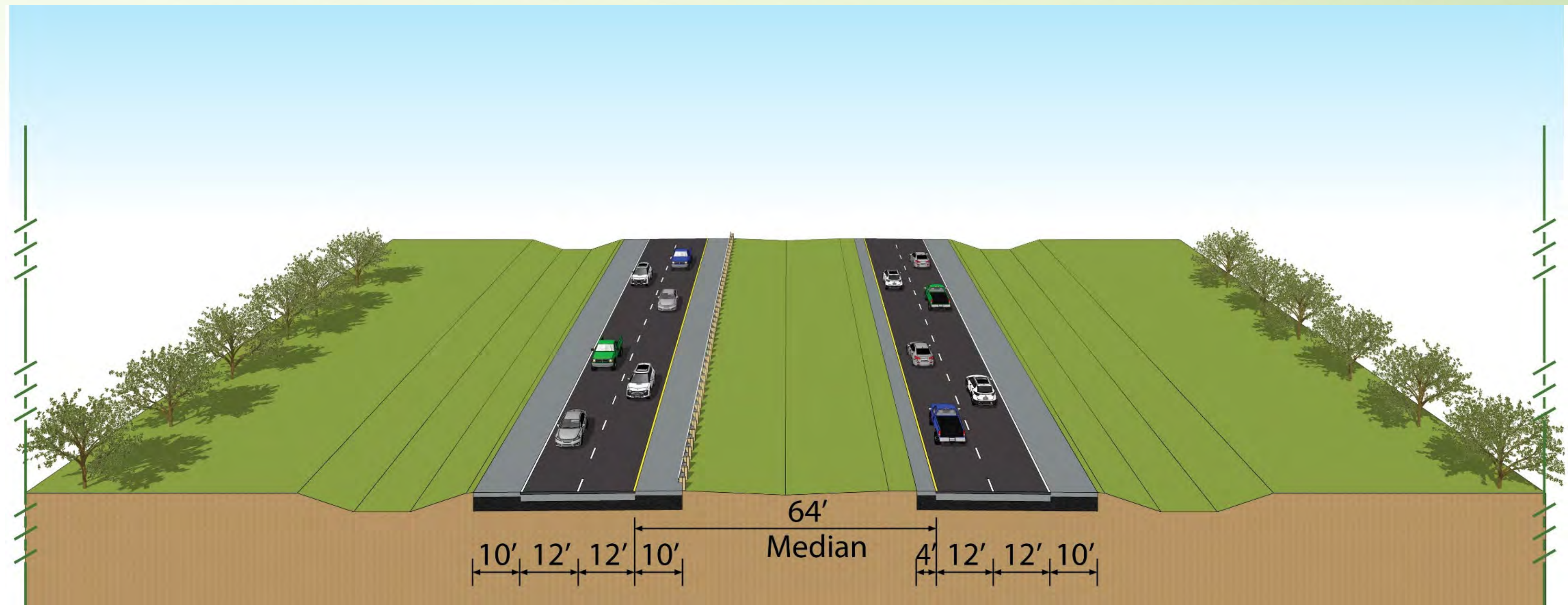
EXISTING ROADWAY TYPICAL SECTION
