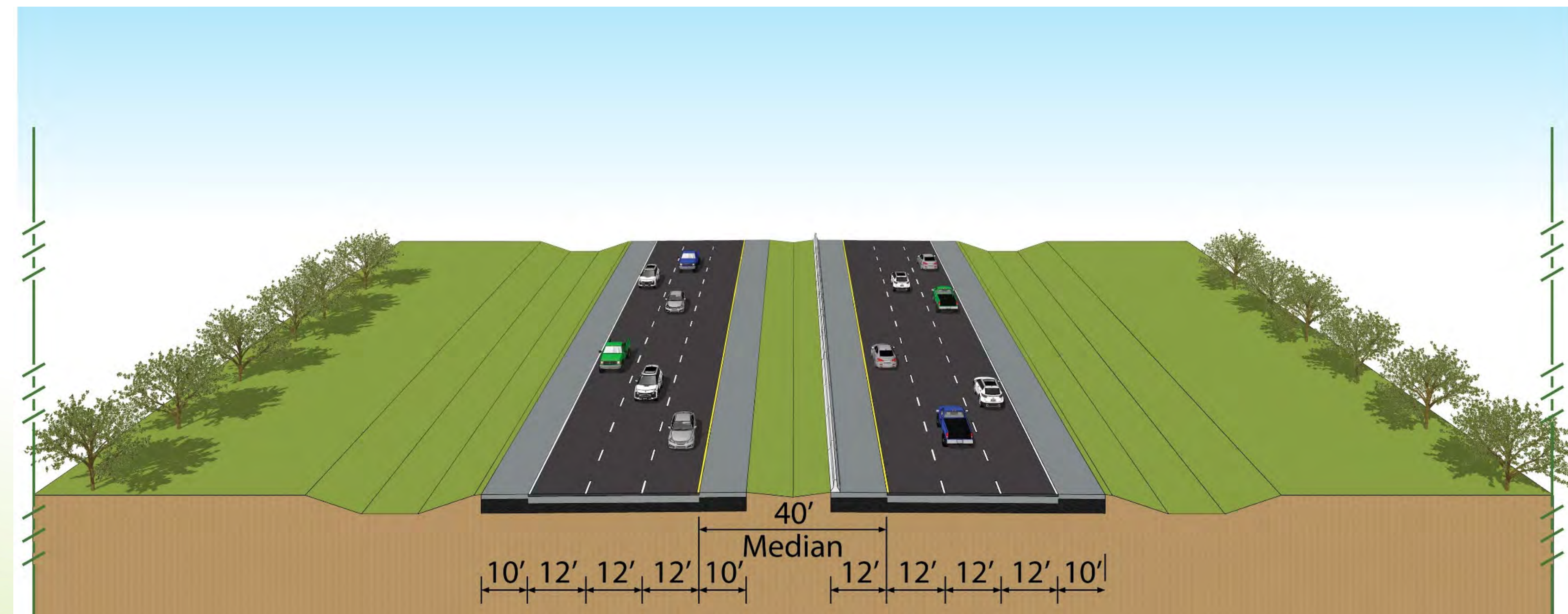
PROPOSED ROADWAY TYPICAL SECTION
